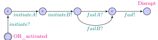
Fig. 9: STA for OR gate and root node of security attack tree.
