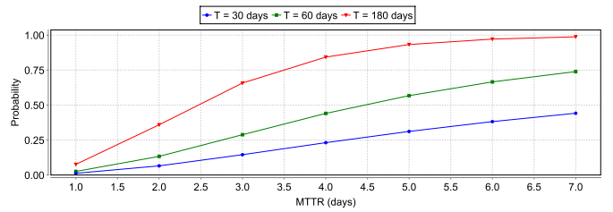
Fig. 4. Disconnection probability for different MTTRs given MTBF
