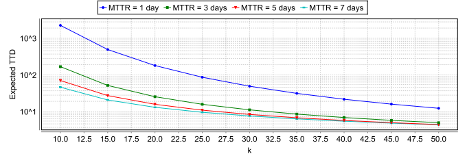
Fig. 7. Expected Time To Disconnection (TTD) for different size of topology with different values of MTTR and MTBF = 60 days
