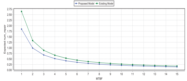
Fig. 8: Maintainability (property 4)
