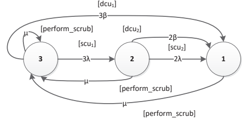
Figure 8: DCU model of TMR with repair
