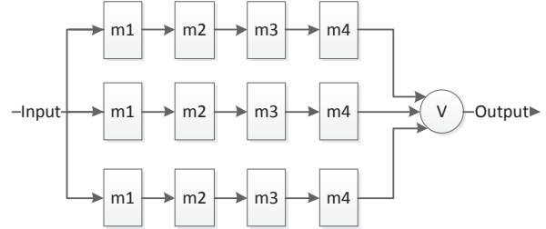
Figure 2: TMR version of the sample circuit
