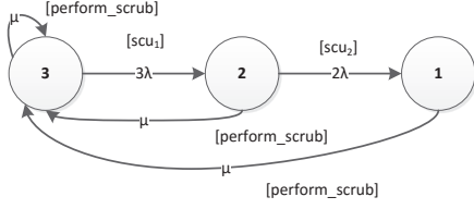
Figure 6: Markov model of TMR with repair
