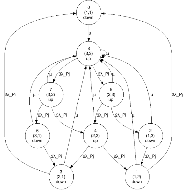
Figure 7: SCU Markov model of TMR with two partitions
